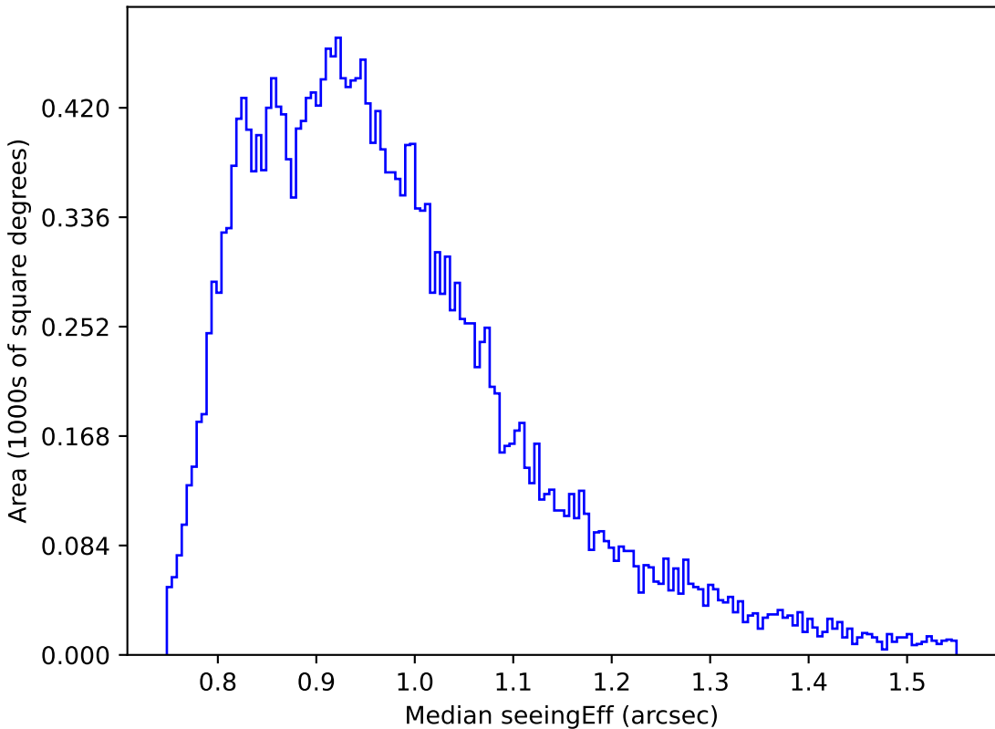
too_elab_r8_d3_ugrizy_v3.4_10yrs Yr 1 r band: Median seeingEff
