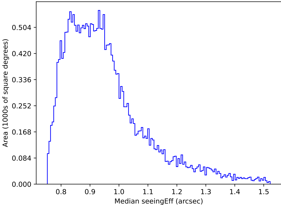
too_elab_r8_d3_ugrizy_v3.4_10yrs Yr 1 i band: Median seeingEff
