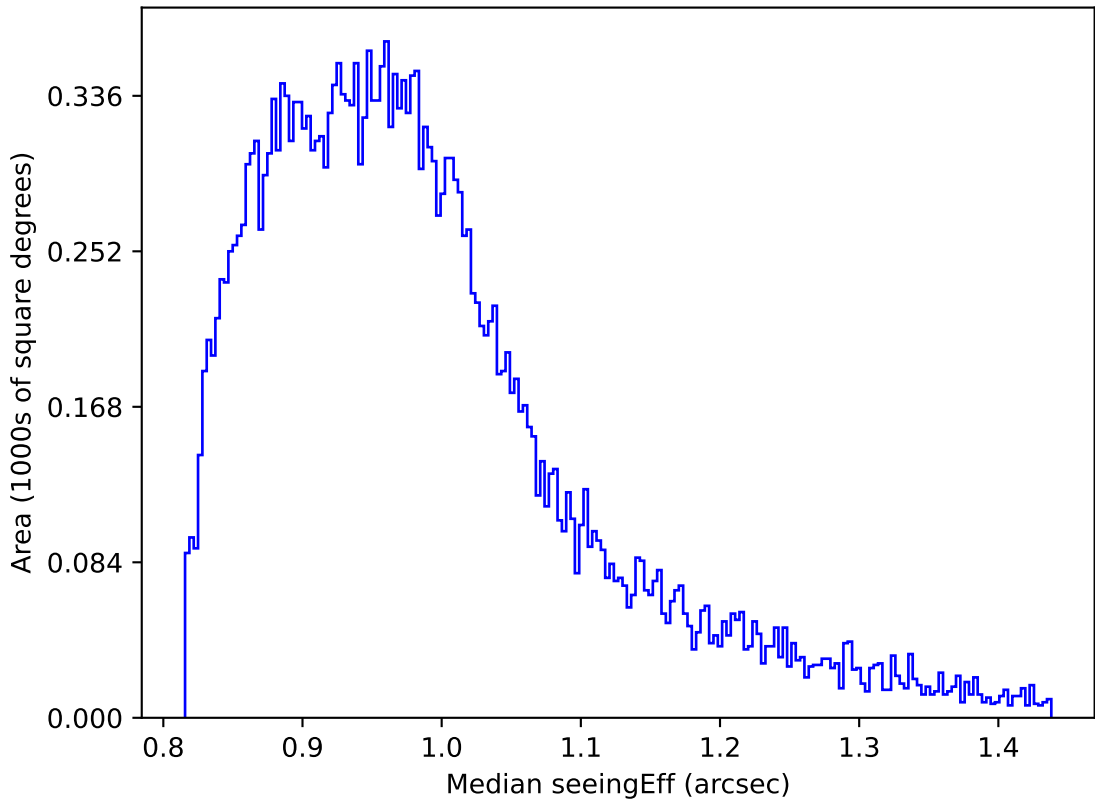
too_elab_r8_d3_ugrizy_v3.4_10yrs Yr 1 all bands: Median seeingEff
