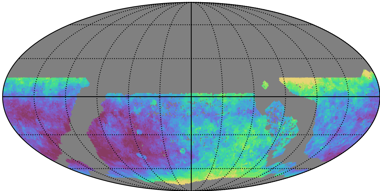
too_elab_r8_d3_ugrizy_v3.4_10yrs WFD z band: Median seeingEff
