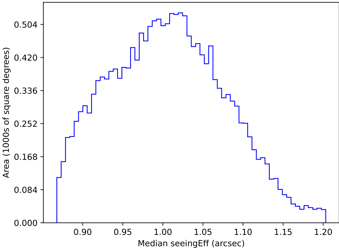
too_elab_r8_d3_ugrizy_v3.4_10yrs WFD z band: Median seeingEff
