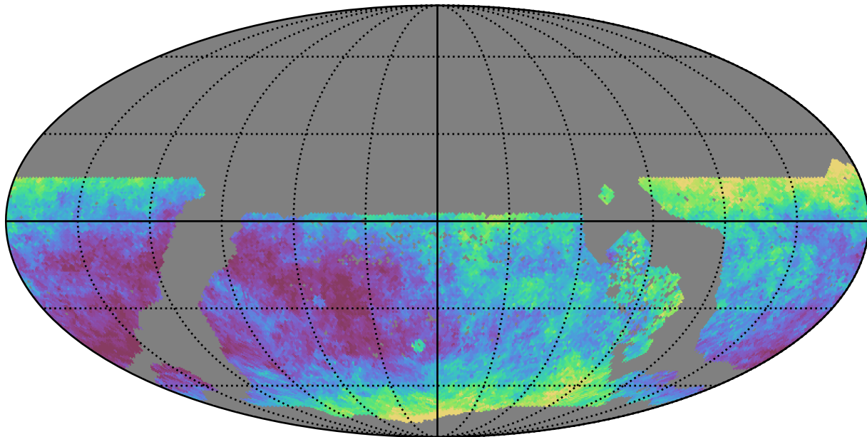
too_elab_r8_d3_ugrizy_v3.4_10yrs WFD y band: Median seeingEff
