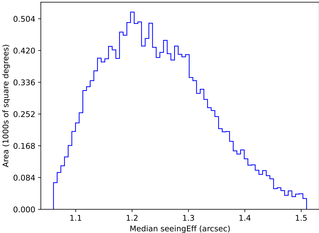
too_elab_r8_d3_ugrizy_v3.4_10yrs WFD u band: Median seeingEff
