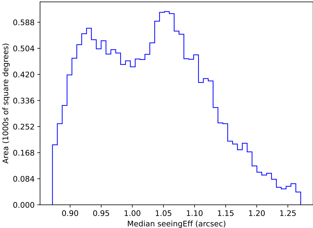
too_elab_r8_d3_ugrizy_v3.4_10yrs WFD r band: Median seeingEff
