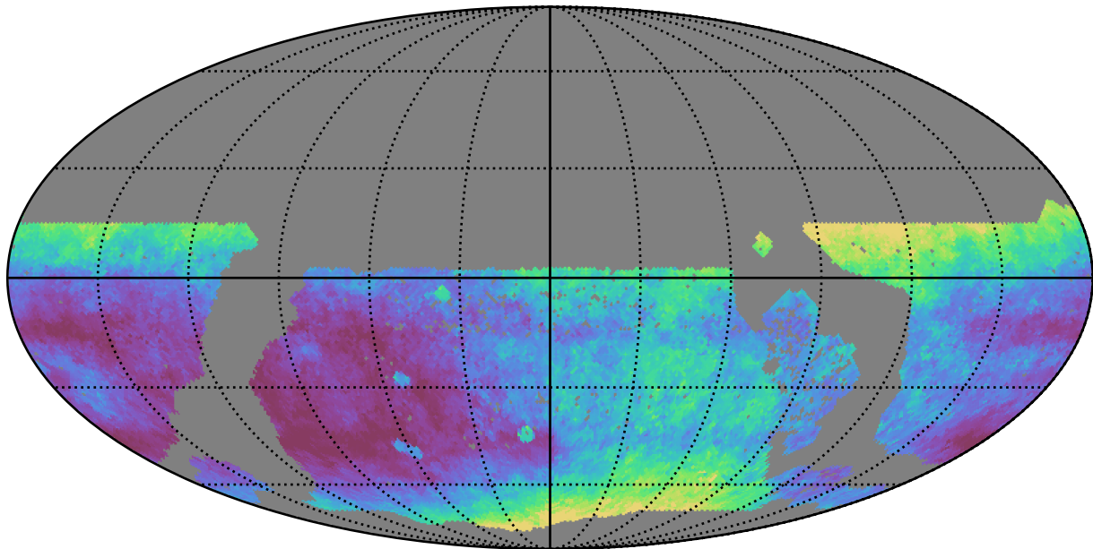
too_elab_r8_d3_ugrizy_v3.4_10yrs WFD i band: Median seeingEff
