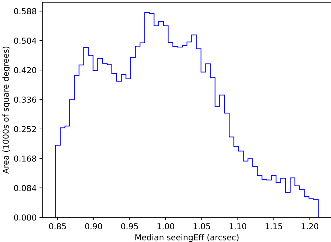
too_elab_r8_d3_ugrizy_v3.4_10yrs WFD i band: Median seeingEff
