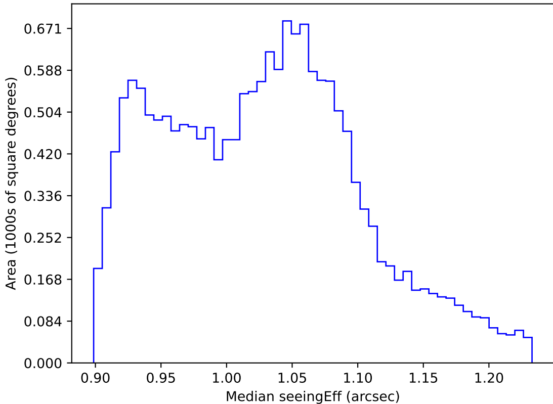
too_elab_r8_d3_ugrizy_v3.4_10yrs WFD all bands: Median seeingEff
