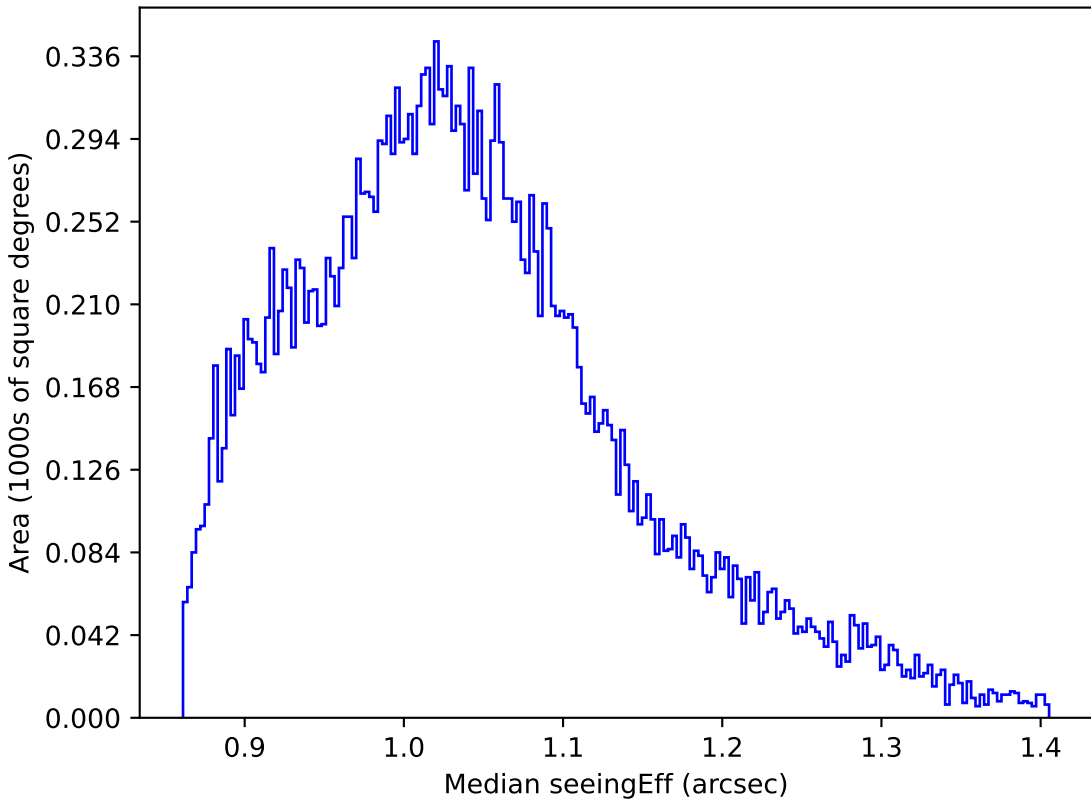
too_elab_r8_d3_ugrizy_v3.4_10yrs All sky z band: Median seeingEff
