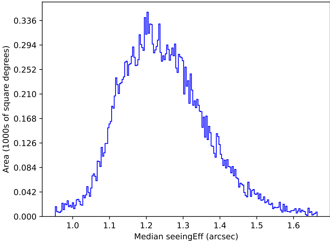
too_elab_r8_d3_ugrizy_v3.4_10yrs All sky u band: Median seeingEff
