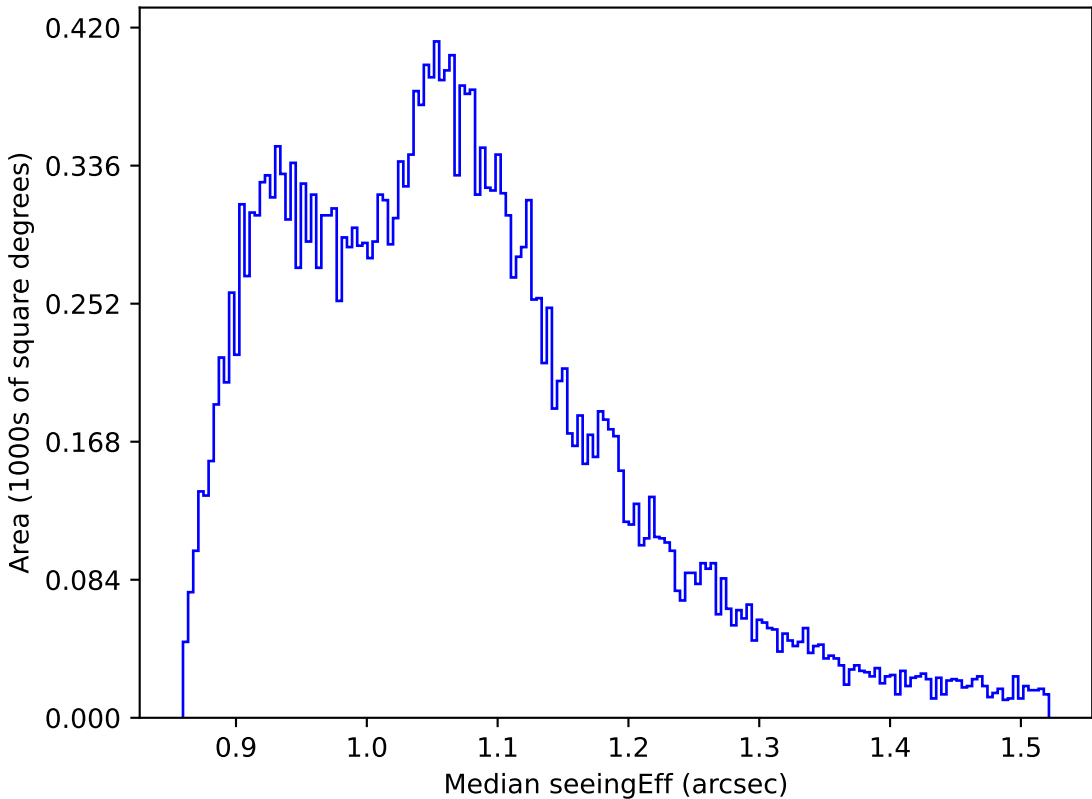
too_elab_r8_d3_ugrizy_v3.4_10yrs All sky r band: Median seeingEff
