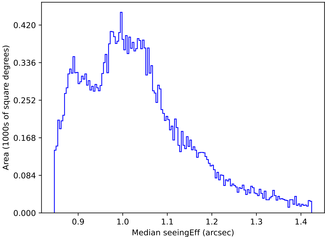
too_elab_r8_d3_ugrizy_v3.4_10yrs All sky i band: Median seeingEff
