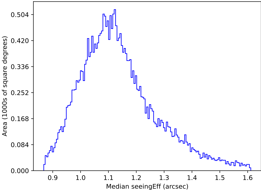
too_elab_r8_d3_ugrizy_v3.4_10yrs All sky g band: Median seeingEff
