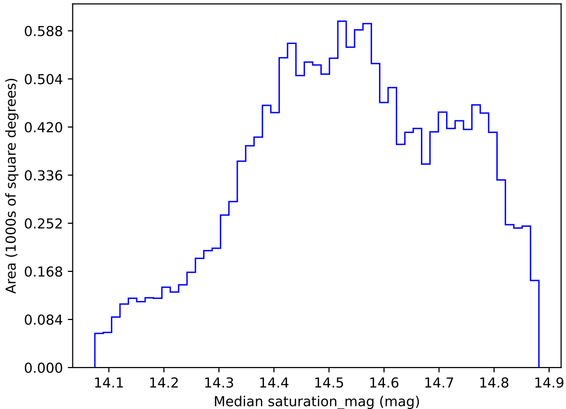
too_elab_r8_d3_ugrizy_v3.4_10yrs WFD i band: Median saturation_mag
