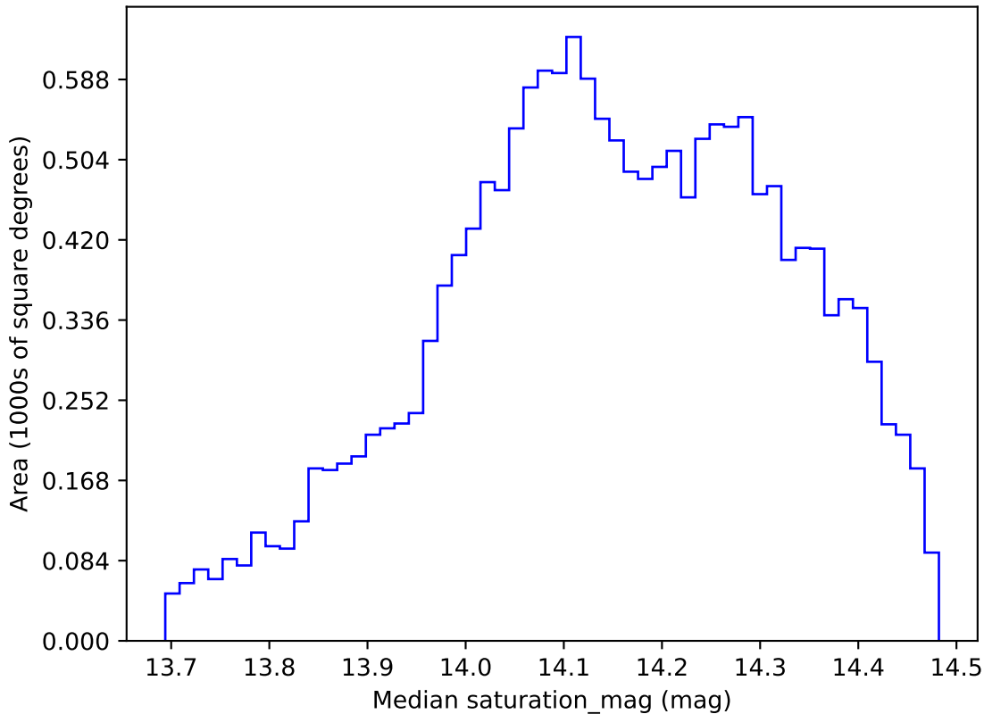
too_elab_r8_d3_ugrizy_v3.4_10yrs WFD all bands: Median saturation_mag
