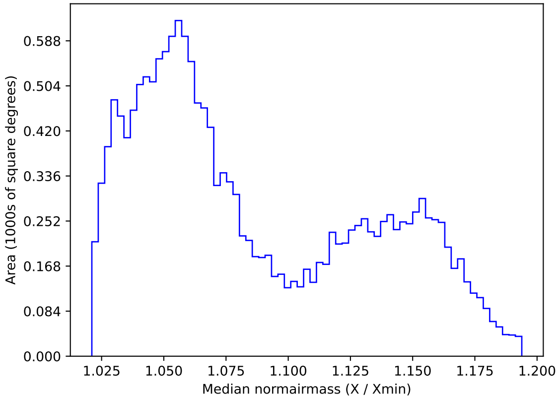
too_elab_r8_d3_ugrizy_v3.4_10yrs WFD z band: Median normairmass
