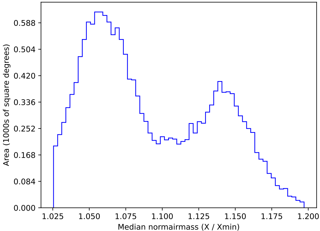
too_elab_r8_d3_ugrizy_v3.4_10yrs WFD y band: Median normairmass
