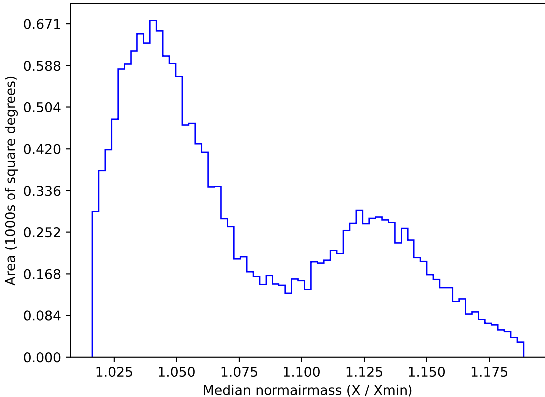
too_elab_r8_d3_ugrizy_v3.4_10yrs WFD r band: Median normairmass
