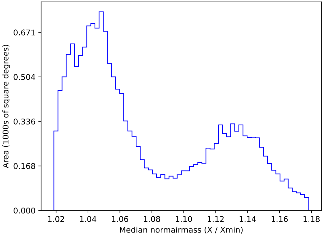
too_elab_r8_d3_ugrizy_v3.4_10yrs WFD i band: Median normairmass
