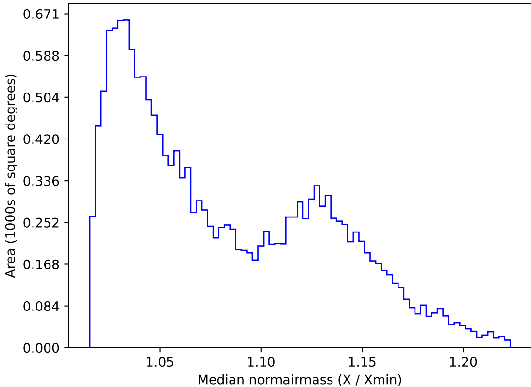
too_elab_r8_d3_ugrizy_v3.4_10yrs WFD g band: Median normairmass
