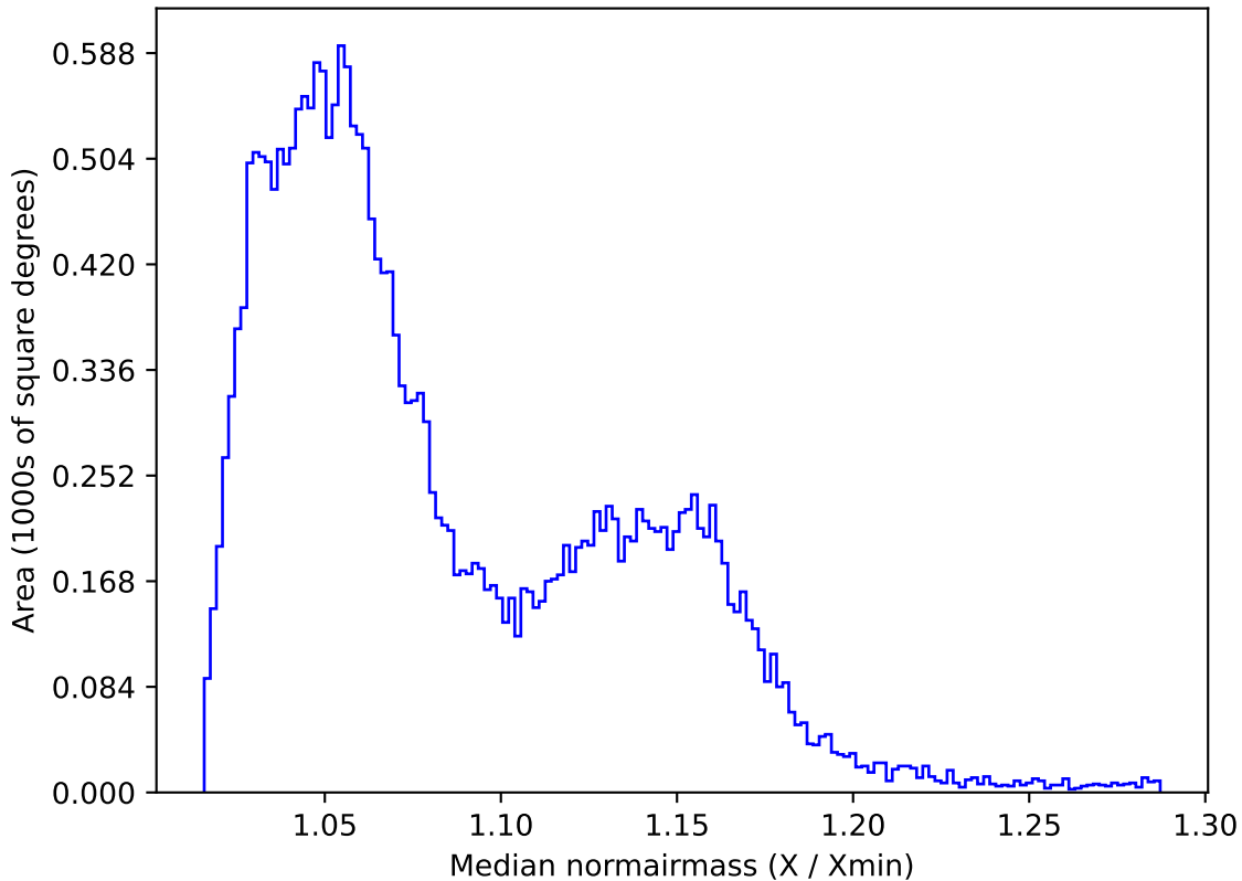
too_elab_r8_d3_ugrizy_v3.4_10yrs All sky z band: Median normairmass
