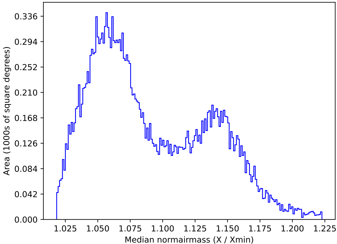
too_elab_r8_d3_ugrizy_v3.4_10yrs All sky y band: Median normairmass
