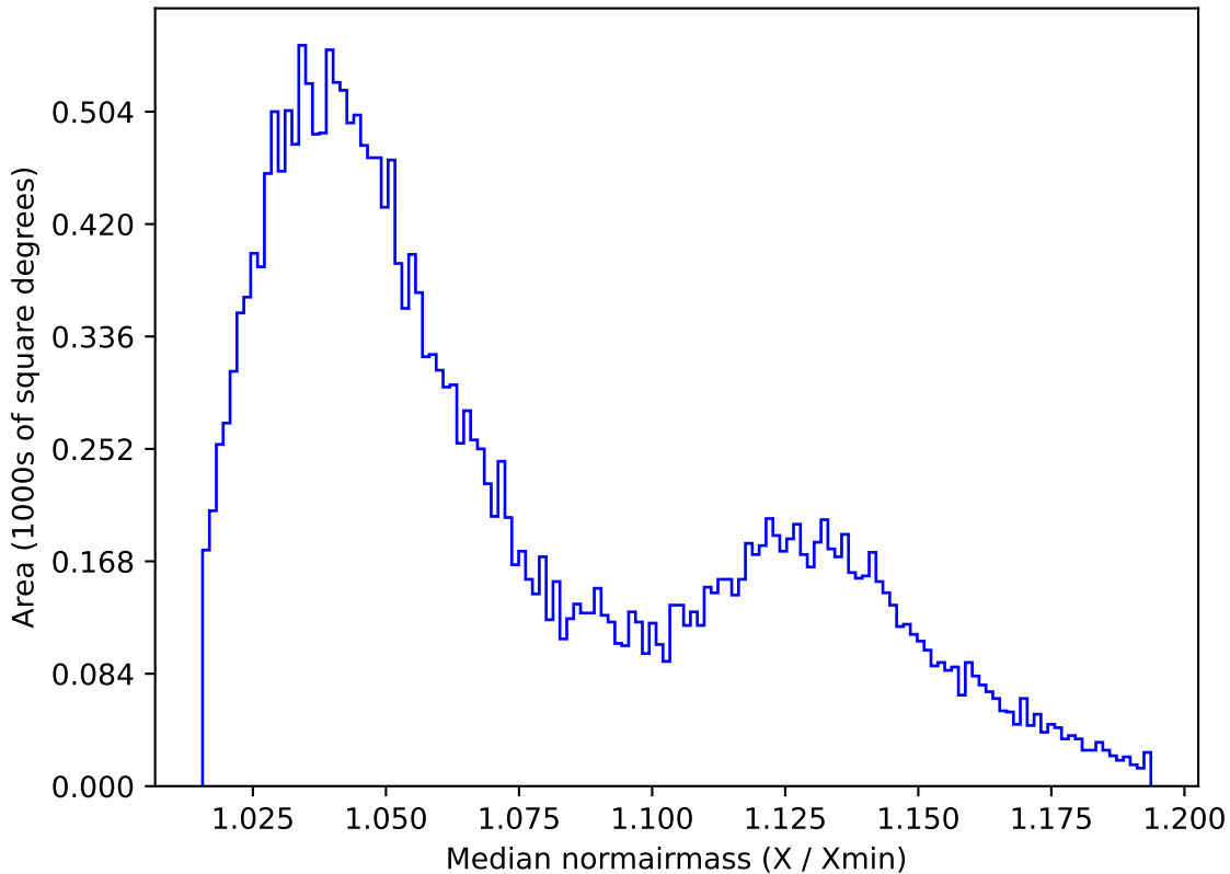
too_elab_r8_d3_ugrizy_v3.4_10yrs All sky r band: Median normairmass
