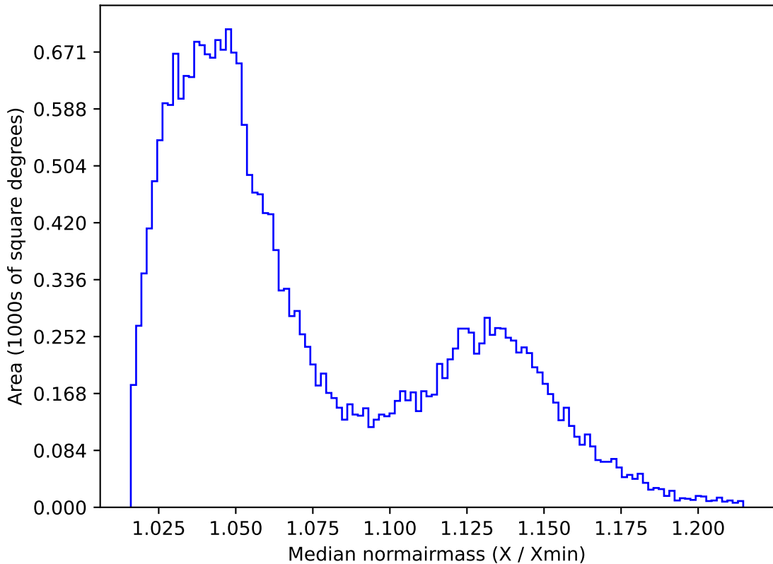
too_elab_r8_d3_ugrizy_v3.4_10yrs All sky i band: Median normairmass
