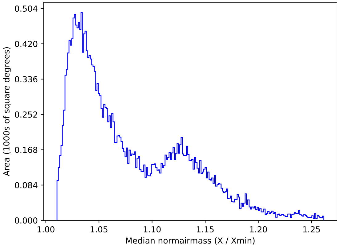
too_elab_r8_d3_ugrizy_v3.4_10yrs All sky g band: Median normairmass
