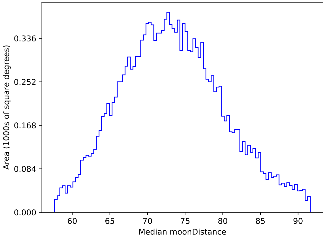
too_elab_r8_d3_ugrizy_v3.4_10yrs WFD z band: Median moonDistance
