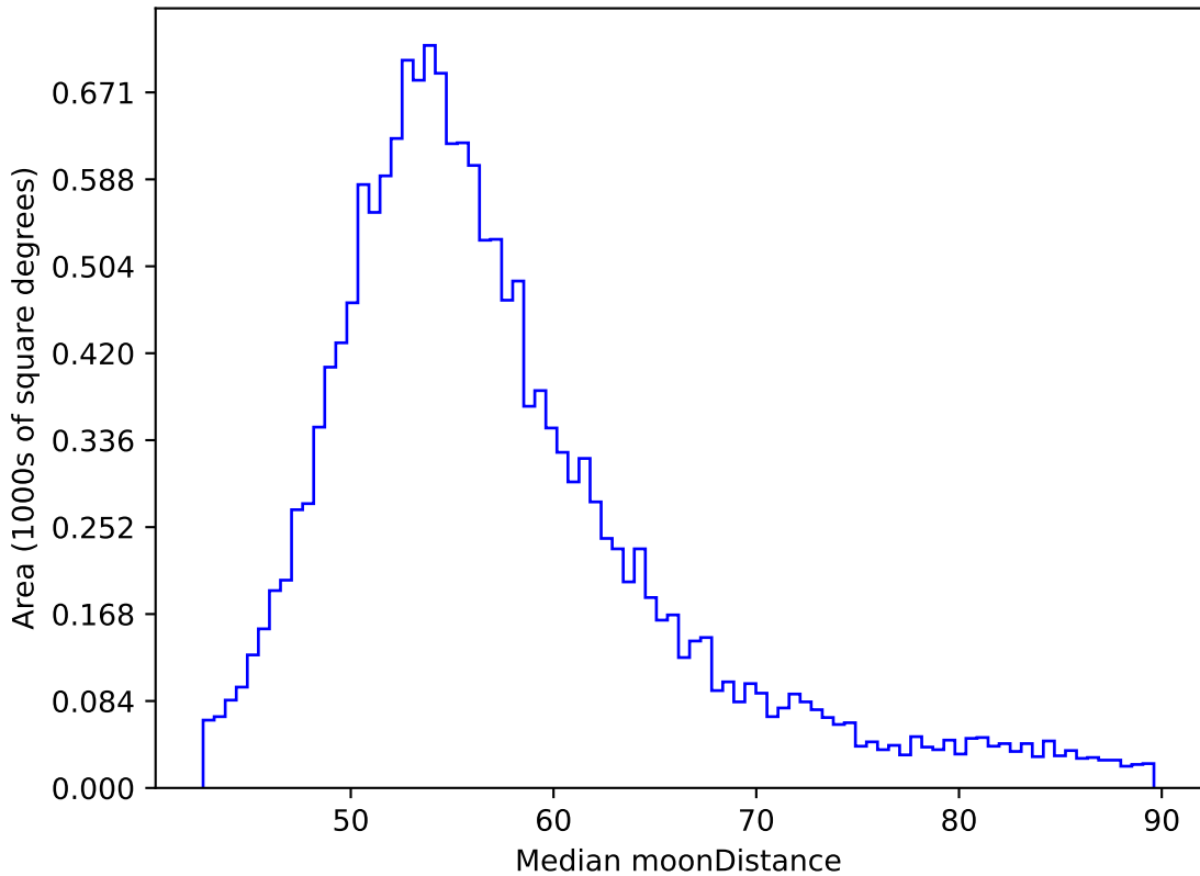
too_elab_r8_d3_ugrizy_v3.4_10yrs WFD y band: Median moonDistance
