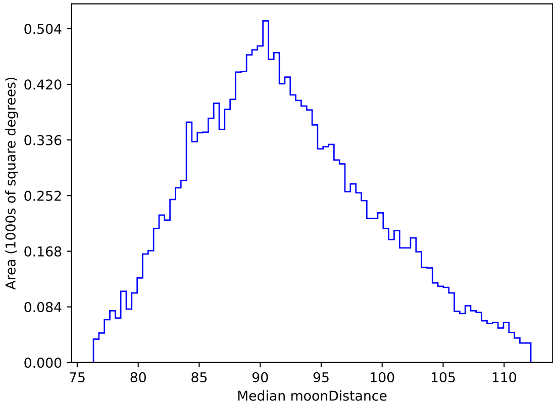
too_elab_r8_d3_ugrizy_v3.4_10yrs WFD i band: Median moonDistance
