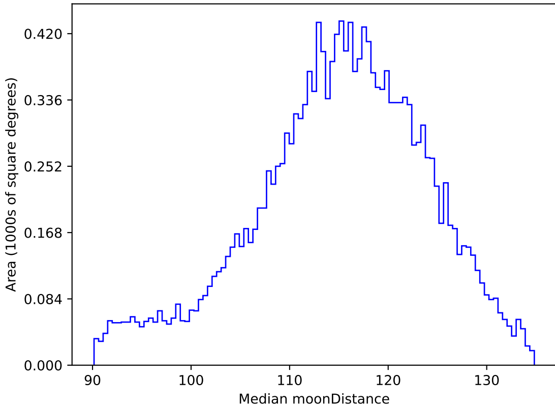
too_elab_r8_d3_ugrizy_v3.4_10yrs WFD g band: Median moonDistance
