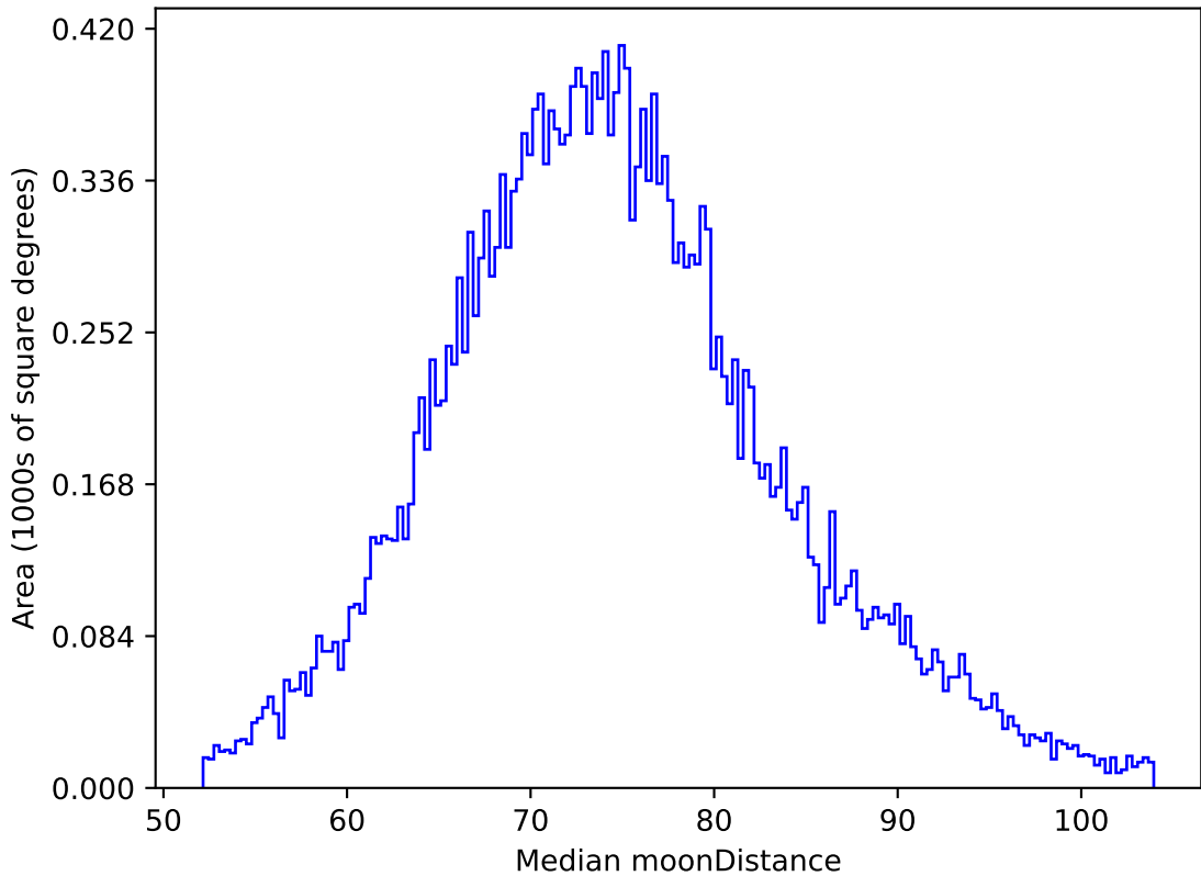
too_elab_r8_d3_ugrizy_v3.4_10yrs All sky z band: Median moonDistance
