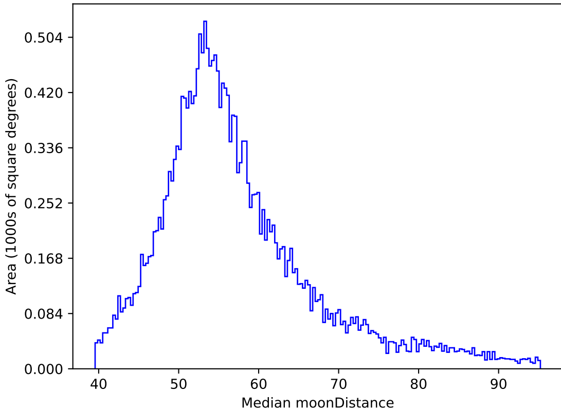
too_elab_r8_d3_ugrizy_v3.4_10yrs All sky y band: Median moonDistance
