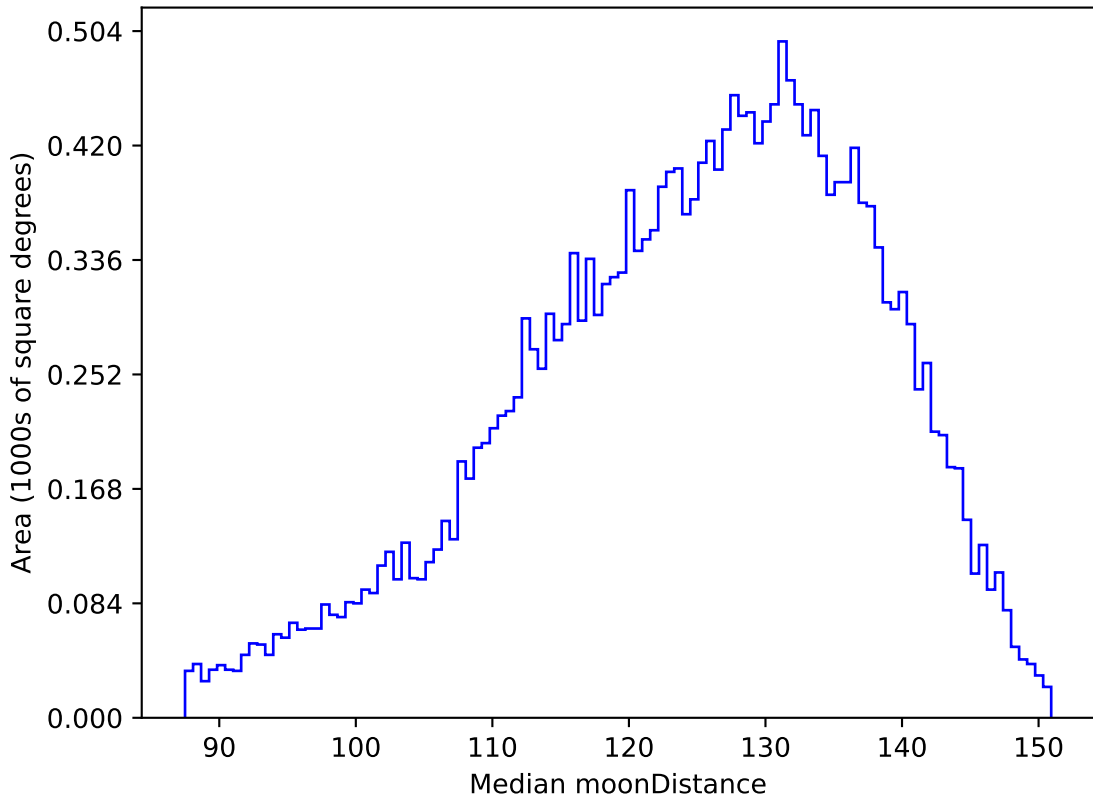
too_elab_r8_d3_ugrizy_v3.4_10yrs All sky u band: Median moonDistance
