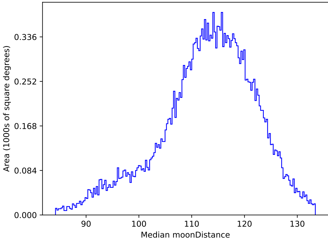
too_elab_r8_d3_ugrizy_v3.4_10yrs All sky r band: Median moonDistance
