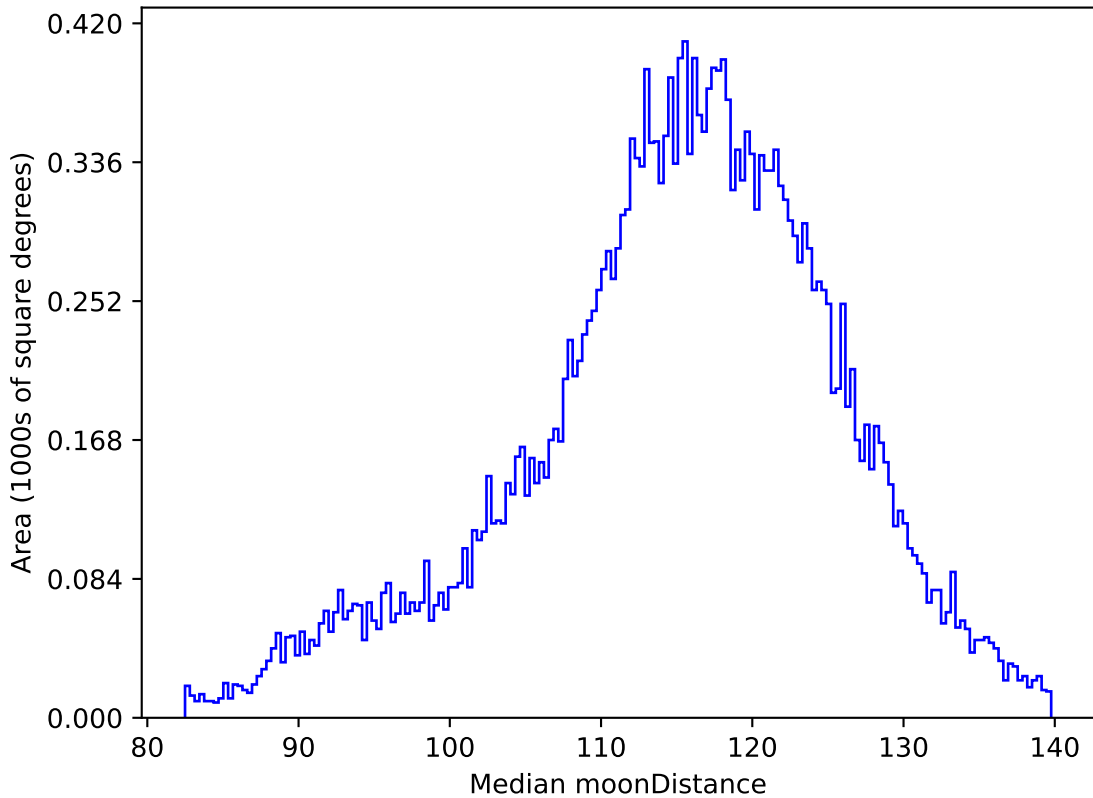
too_elab_r8_d3_ugrizy_v3.4_10yrs All sky g band: Median moonDistance
