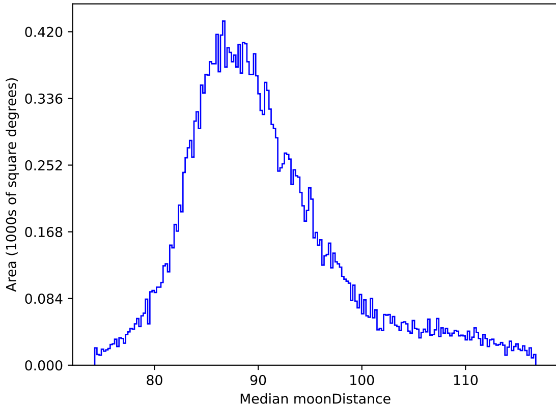
too_elab_r8_d3_ugrizy_v3.4_10yrs All sky all bands: Median moonDistance
