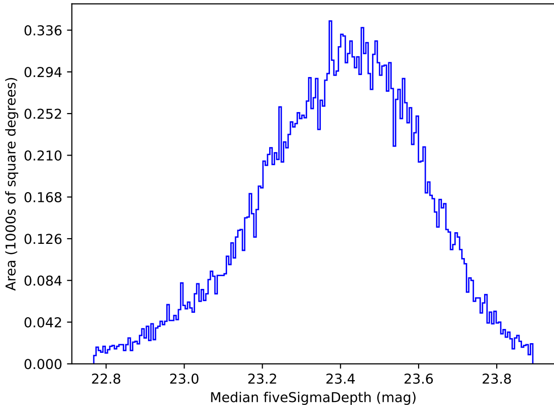
too_elab_r8_d3_ugrizy_v3.4_10yrs Yr 1 all bands: Median fiveSigmaDepth
