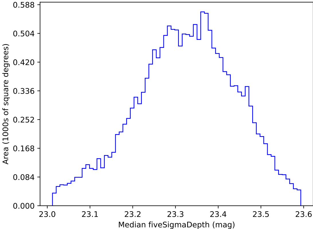
too_elab_r8_d3_ugrizy_v3.4_10yrs WFD all bands: Median fiveSigmaDepth
