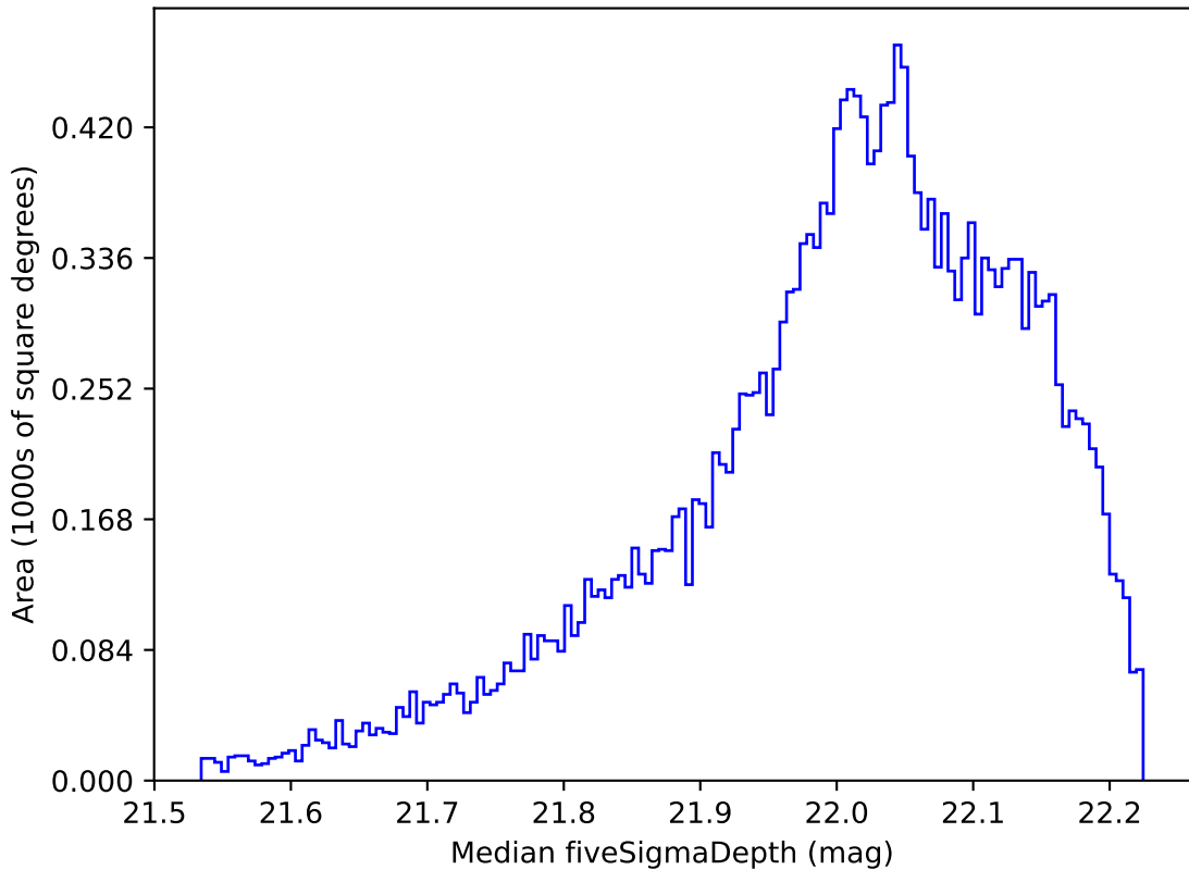
too_elab_r8_d3_ugrizy_v3.4_10yrs All sky y band: Median fiveSigmaDepth
