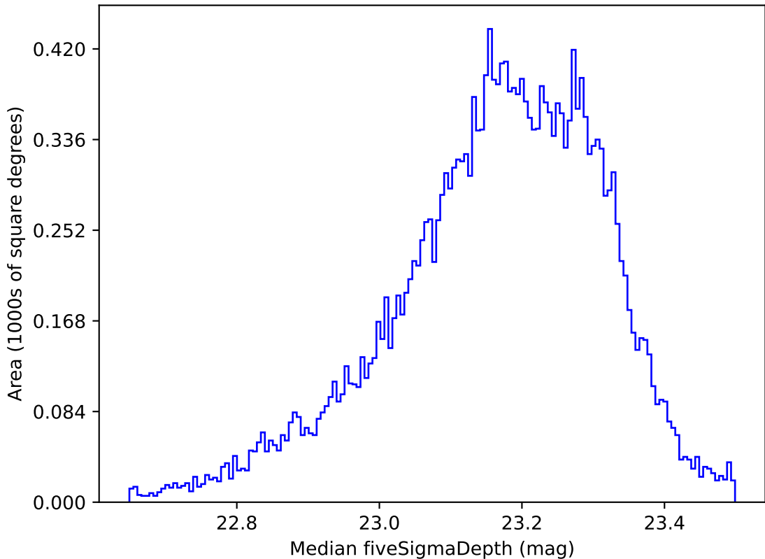
too_elab_r8_d3_ugrizy_v3.4_10yrs All sky u band: Median fiveSigmaDepth
