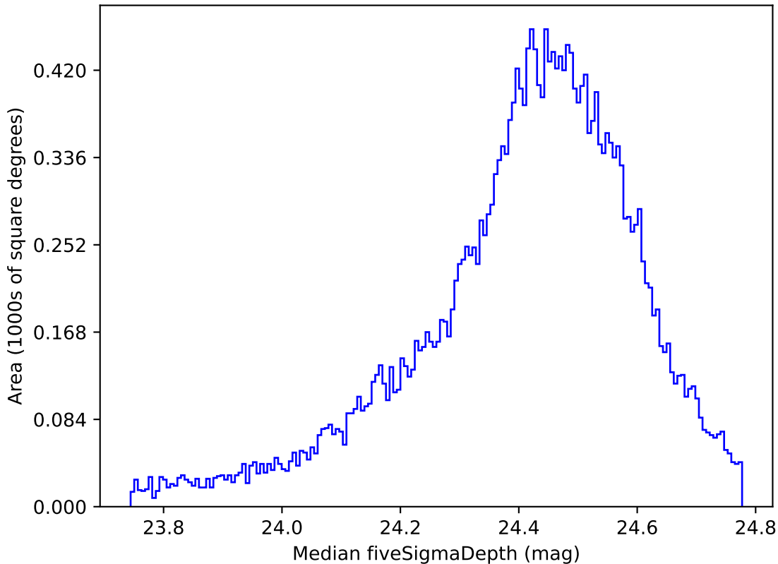
too_elab_r8_d3_ugrizy_v3.4_10yrs All sky g band: Median fiveSigmaDepth
