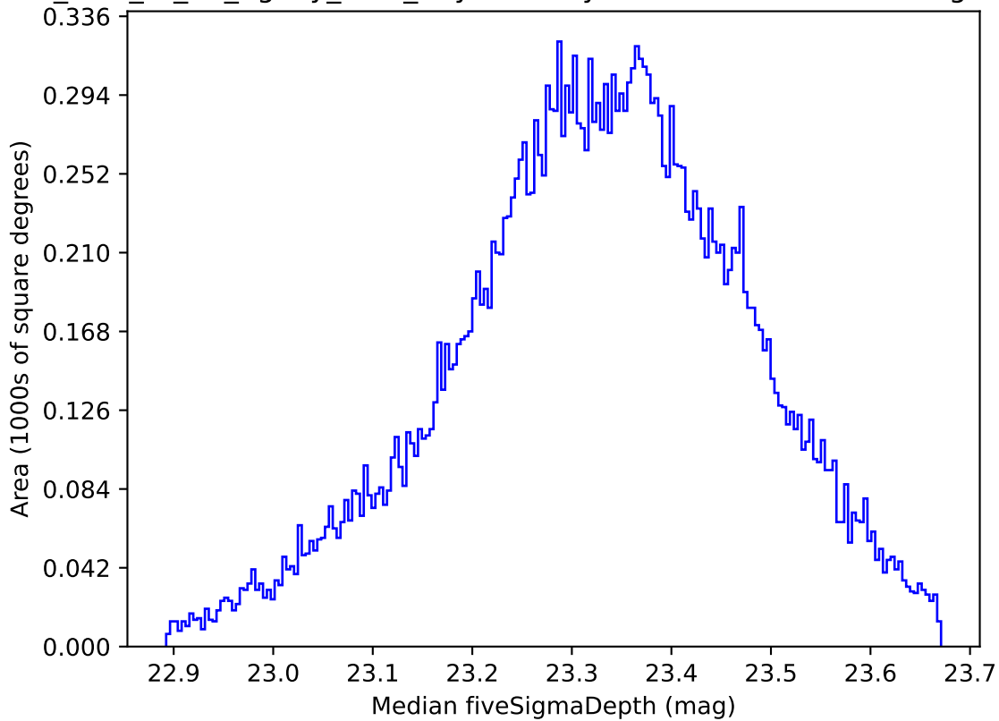
too_elab_r8_d3_ugrizy_v3.4_10yrs All sky all bands: Median fiveSigmaDepth
