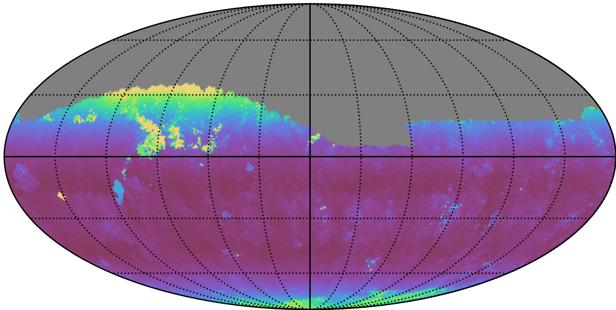
too_elab_r8_d3_ugrizy_v3.4_10yrs Yr 1 z band: Median airmass
