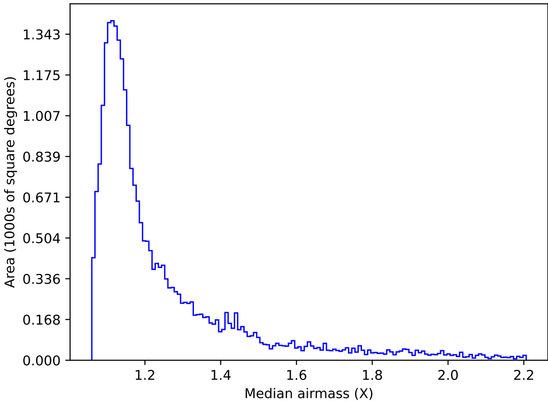
too_elab_r8_d3_ugrizy_v3.4_10yrs Yr 1 z band: Median airmass
