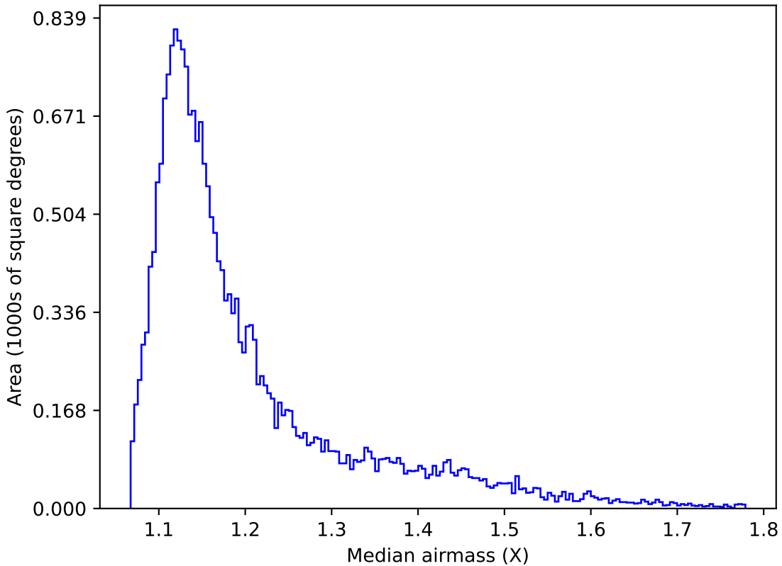
too_elab_r8_d3_ugrizy_v3.4_10yrs Yr 1 y band: Median airmass
