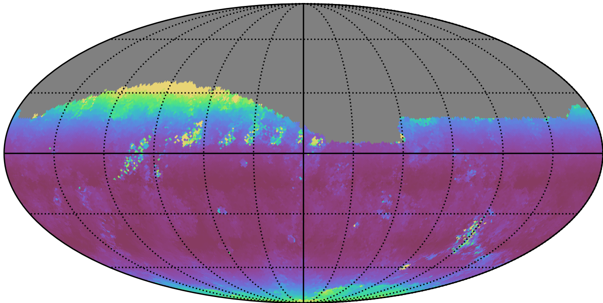
too_elab_r8_d3_ugrizy_v3.4_10yrs Yr 1 r band: Median airmass
