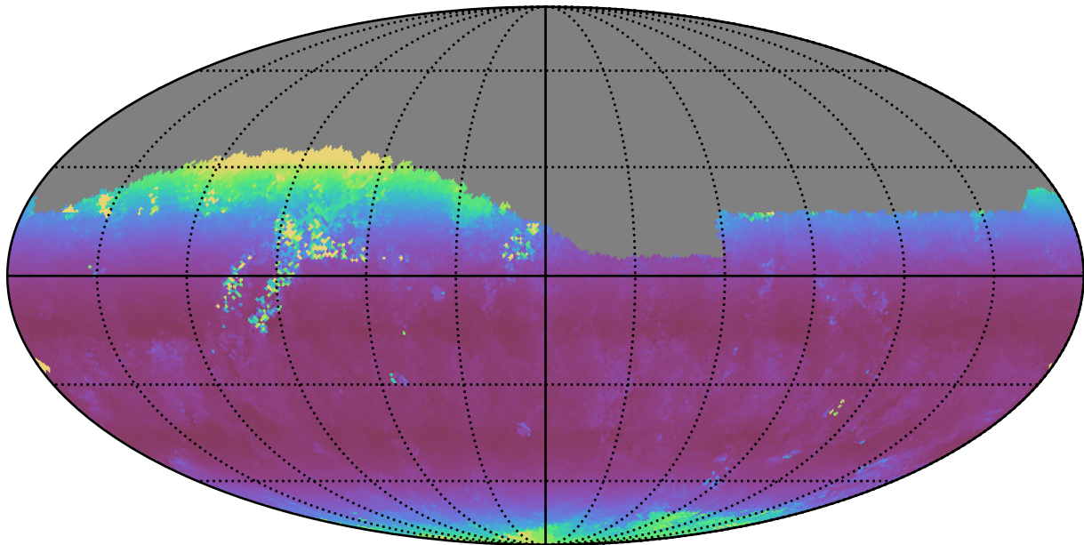
too_elab_r8_d3_ugrizy_v3.4_10yrs Yr 1 i band: Median airmass
