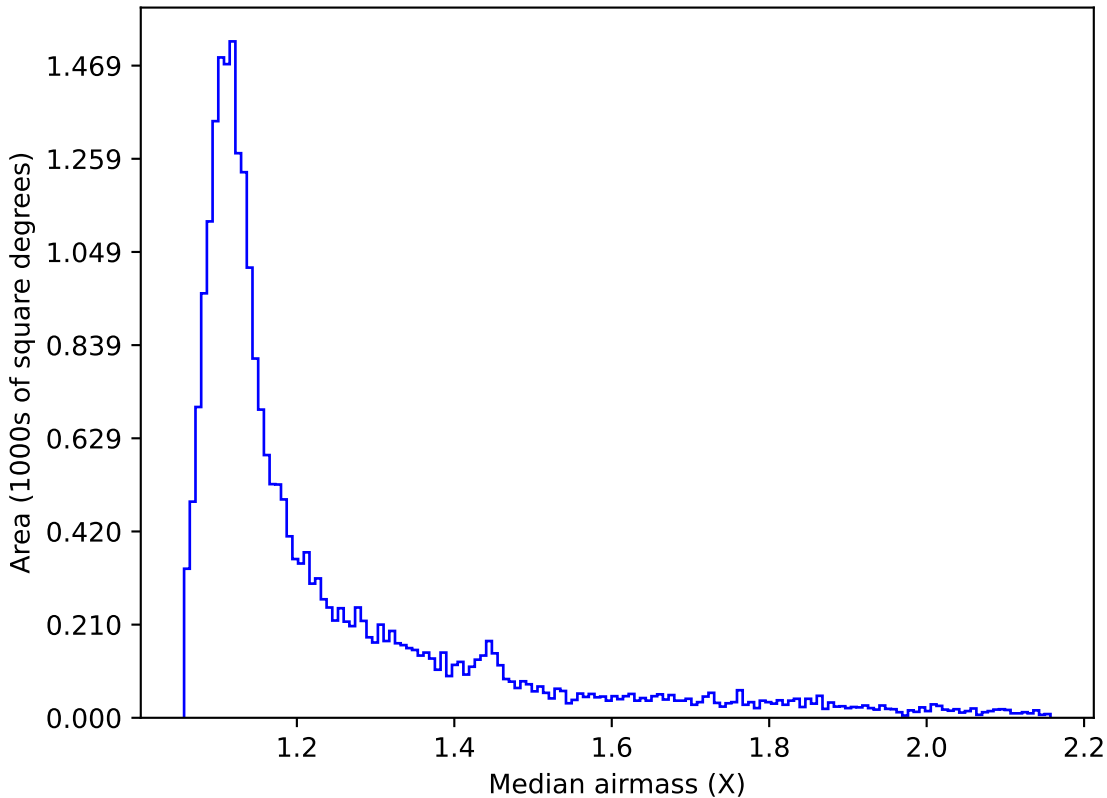
too_elab_r8_d3_ugrizy_v3.4_10yrs Yr 1 i band: Median airmass
